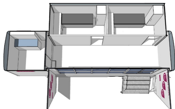
Interior plan showing reception area, two full-size scanning rooms plus additional consultation room
